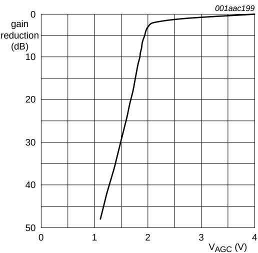
V_{DS(B)} = 5 V; V_{GG} = 5 V; V_{DS(A)} = V_{G1-S(A)} = 0 V; R_{G1} = 150 k \Omega (connected to V_{GG} ); f = 50 MHz; T_{amb} = 25 °C; see Figure 34 .
