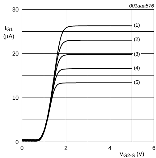
(1) V_{GG} = 5.0 V. (2) V_{GG} = 4.5 V. (3) V_{GG} = 4.0 V. (4) V_{GG} = 3.5 V. (5) V_{GG} = 3.0 V. V_{DS(B)} = 5 V; V_{DS(A)} = V_{G1-S(A)} = 0 V; T_j = 25 °C; R_{G1} = 150 k \Omega (connected to V_{GG} ); see Figure 3 .
